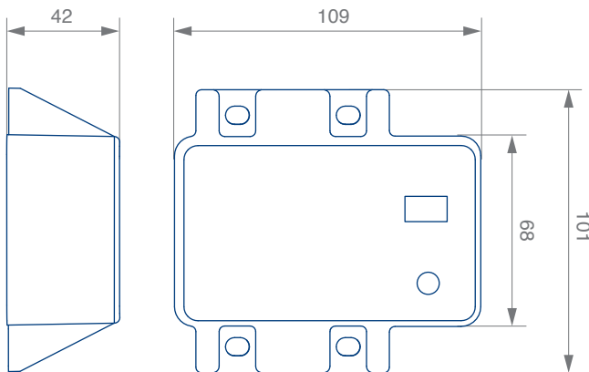
Ref. 432028 Measurements in mm
